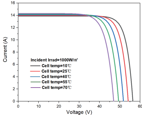
I-V characteristics at different temperatures (SP-M10/156H600W)
