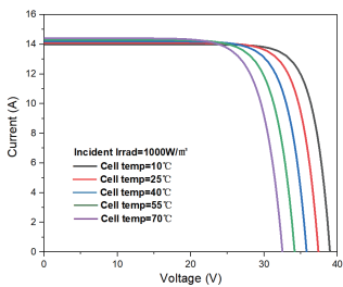
I-V characteristics at different temperatures (SP-M10/108HG415W)
