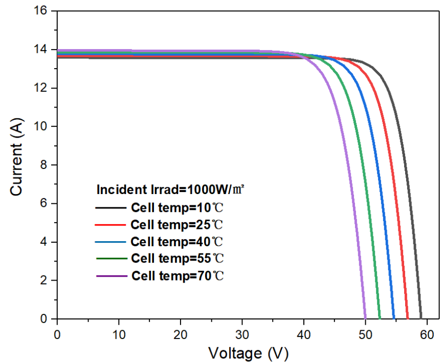
I-V Curves of SP-N16/156HG640W at different cell temperature
