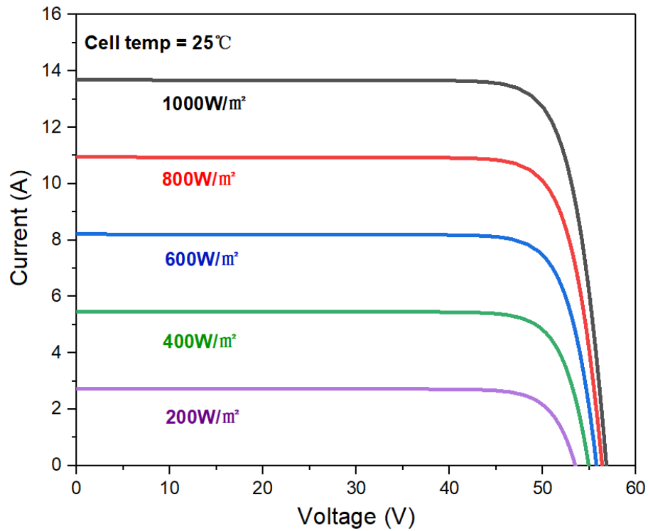
I-V Curves of SP-N16/156HG640W at different irradiance
