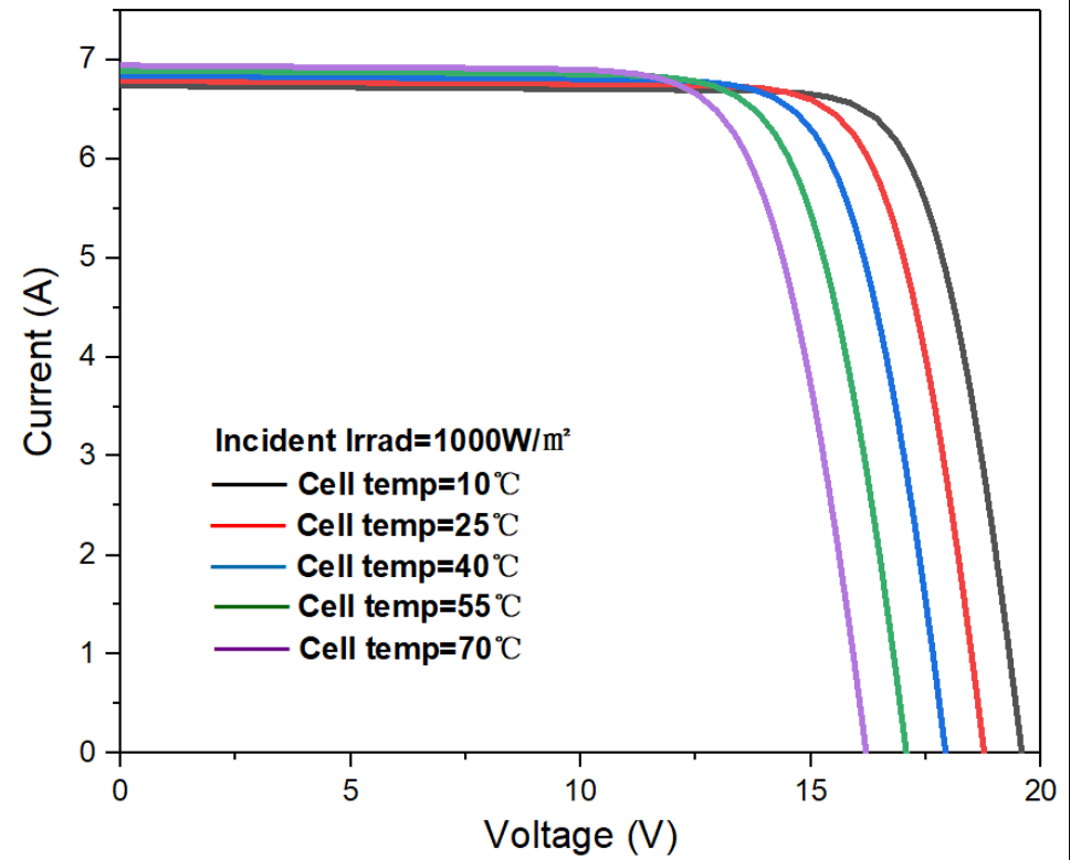
I-V Curves of SP-M10/27H100W at different cell temperature
