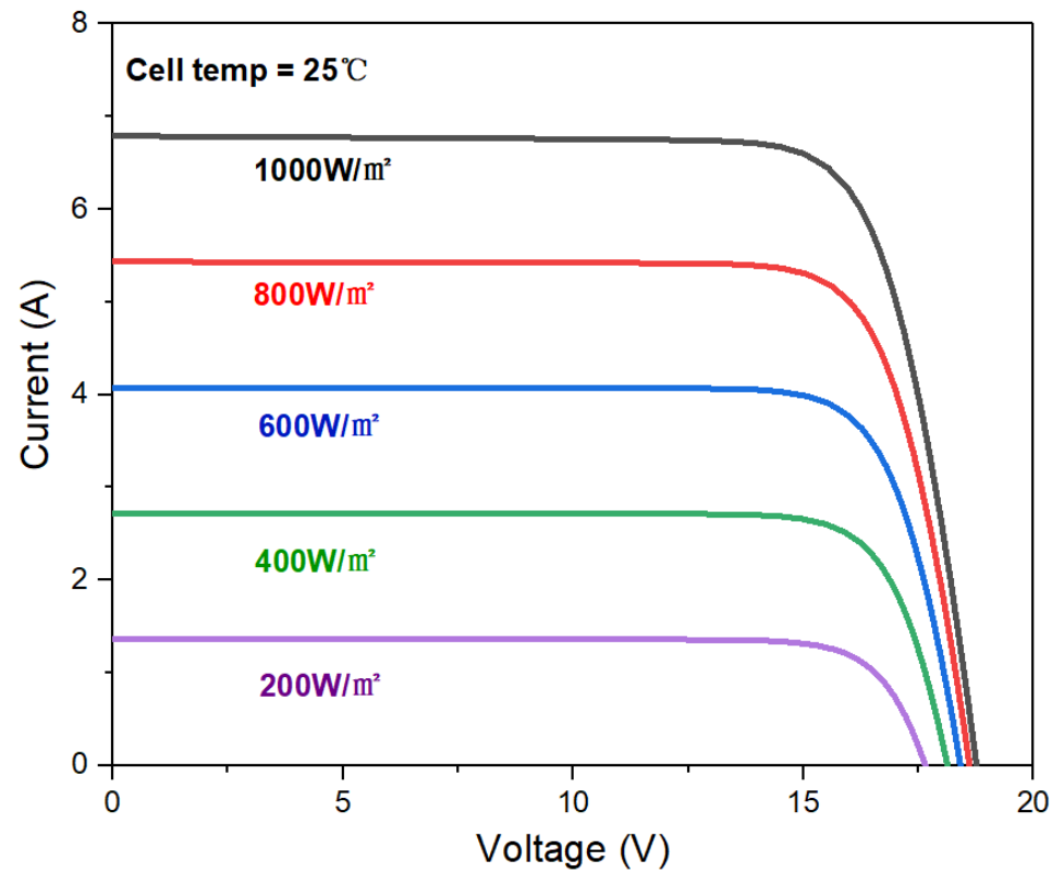
I-V Curves of SP-M10/27H100W at different irradiance
