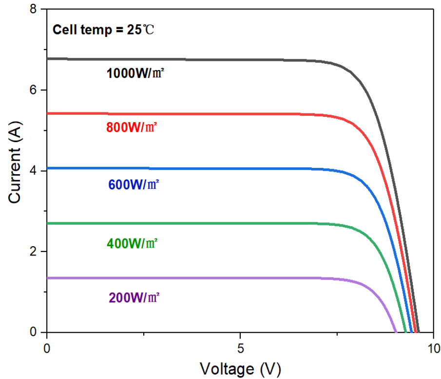
I-V Curves of SP-M10/14H50W at different irradiance
