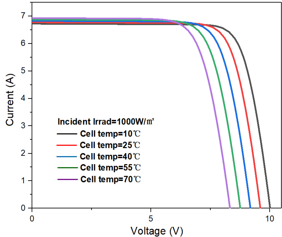
I-V Curves of SP-M10/14H50W at different cell temperature
