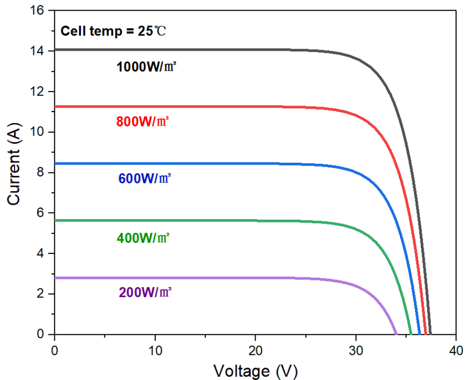
I-V Curves of SP-M10/108H415W at different irradiance
