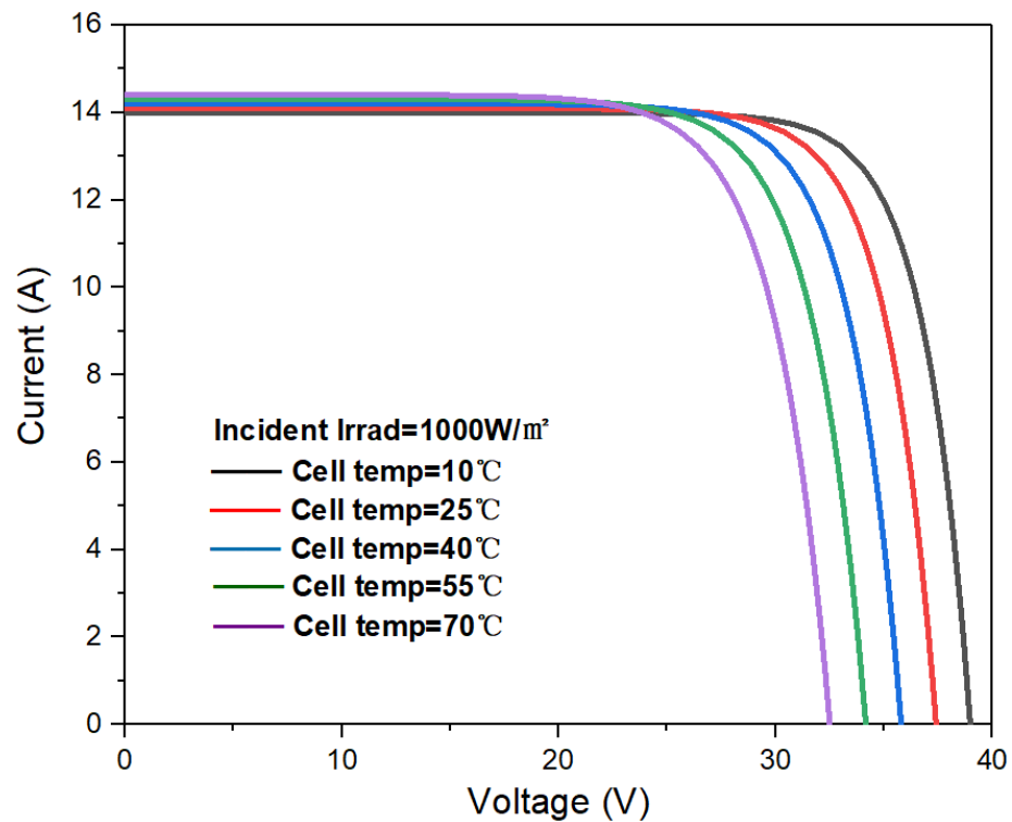
I-V Curves of SP-M10/108H415W at different cell temperature
